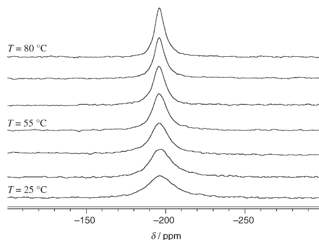
Figure 1. 36.1 MHz 14 N NMR spectra of 5 dissolved in EtOH. The temperature is increased in 10 °C steps, except for the last one (5 °C).
