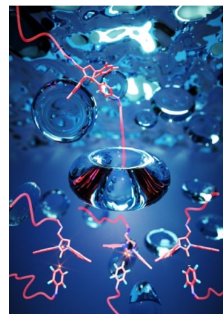
Figure 1. Cartoon depiction of the cavitation-induced mechanical activation of a mechanophore breaking along three concomitant dissociation pathways. 1-2
