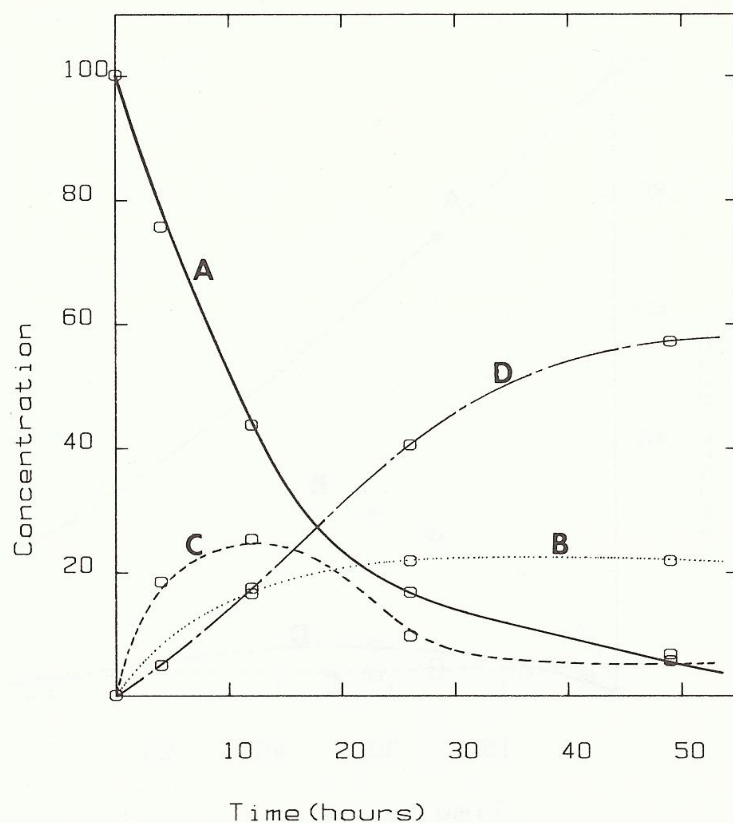
FIGURE 4 Time course for the reaction between AMP and fluorofumarate as catalyzed by argininosuccinate lyase. (A) Fluorofumarate. (B) Intermediate. (C) Oxalacetate (D) Pyruvate. Additional details are given in the text.
