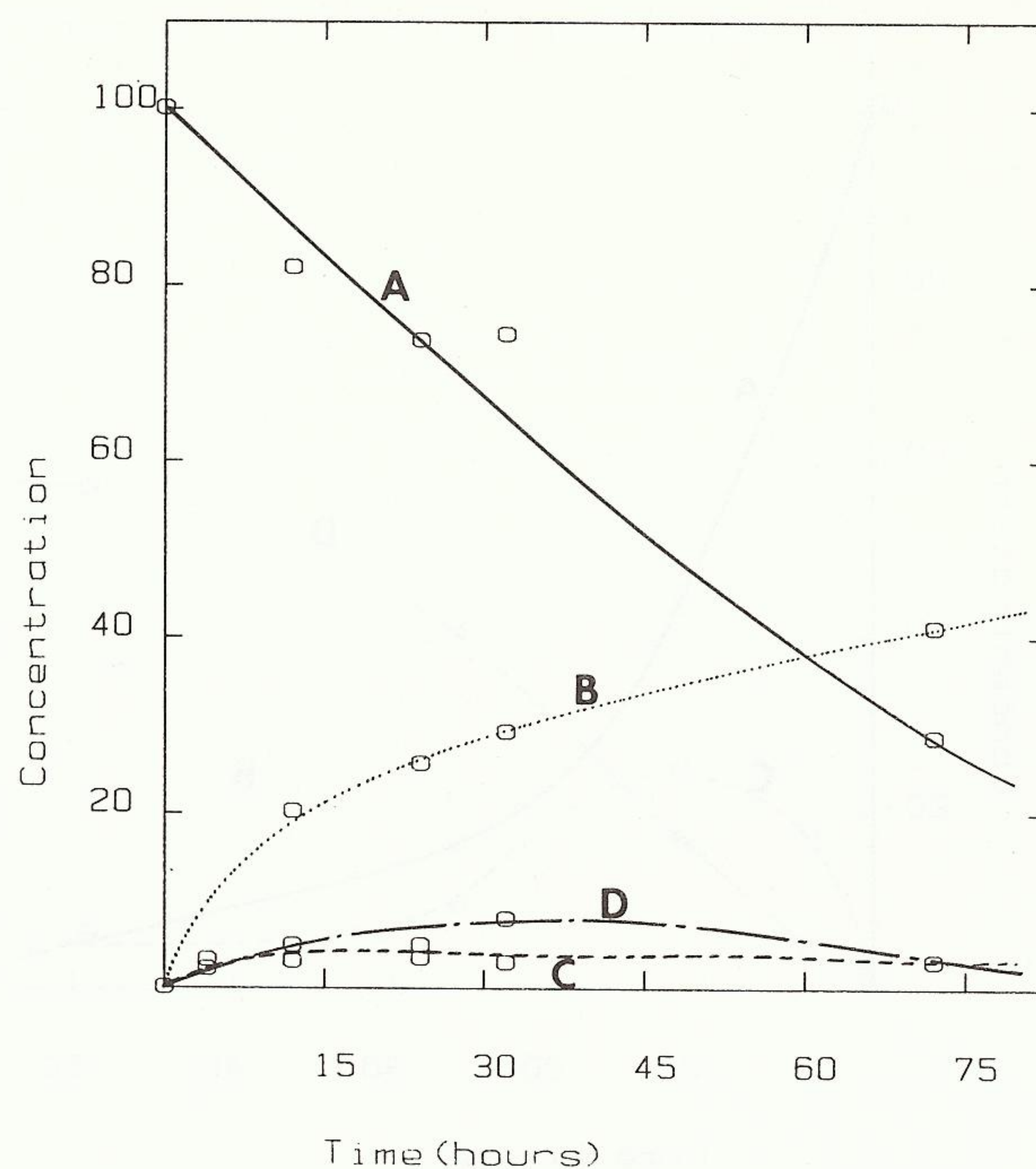
FIGURE 3 Time course for the reaction between AICAR and fluorofumarate as catalyzed by argininosuccinate lyase. (A) Fluorofumarate. (B) Intermediate. (C) Oxalacetate (D) Pyruvate. Additional details are given in the text.
